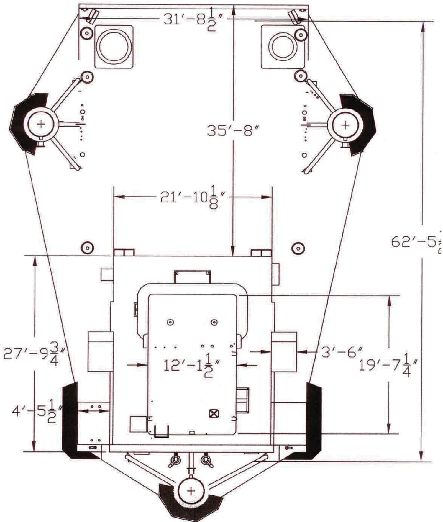
OVERHEAD PROFILE
